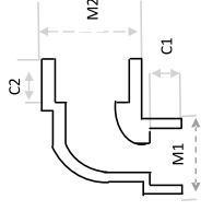
Elbow 90°
